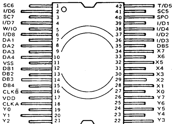
GPKD Pin Configuration
