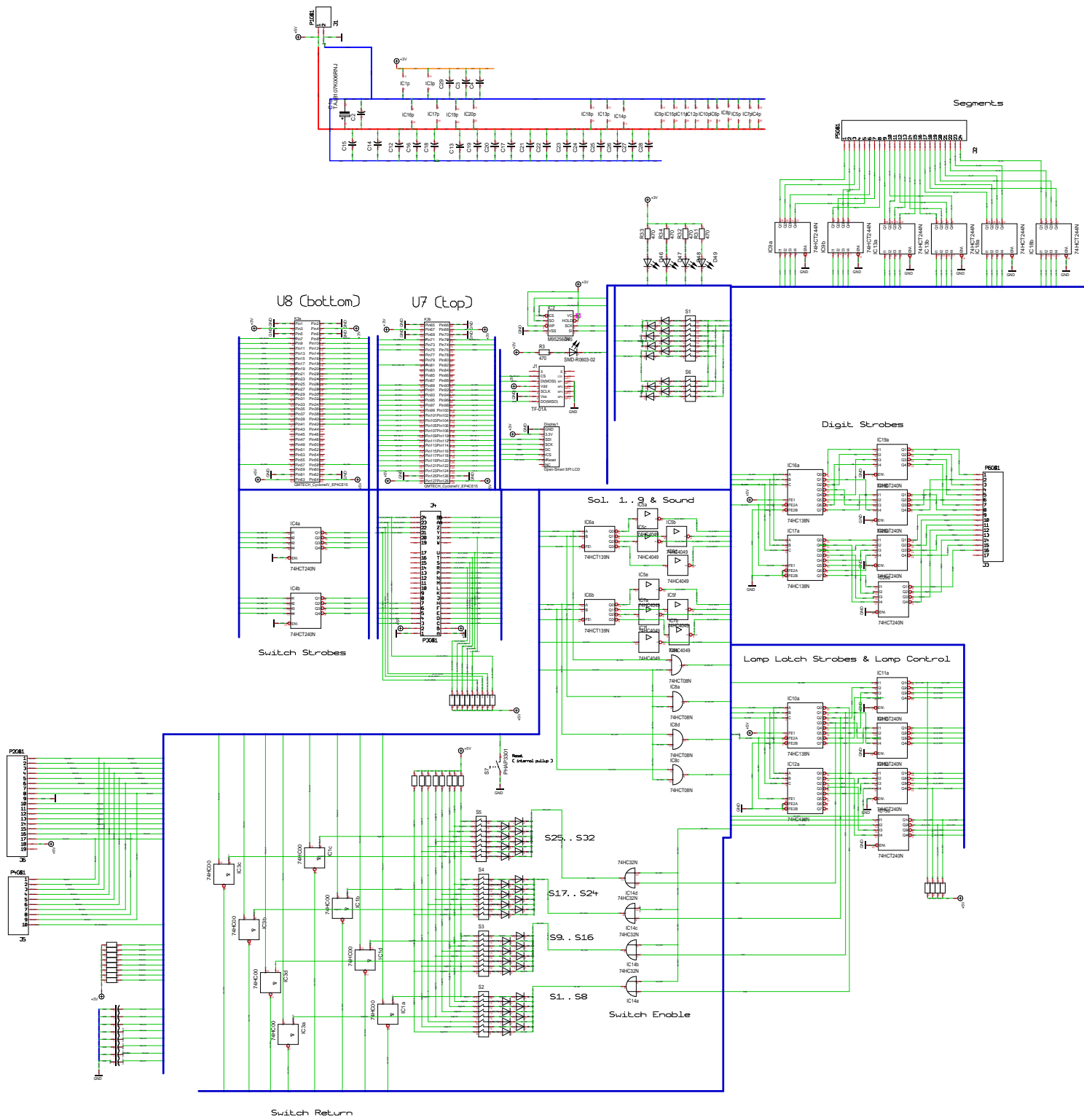
Switch Return
